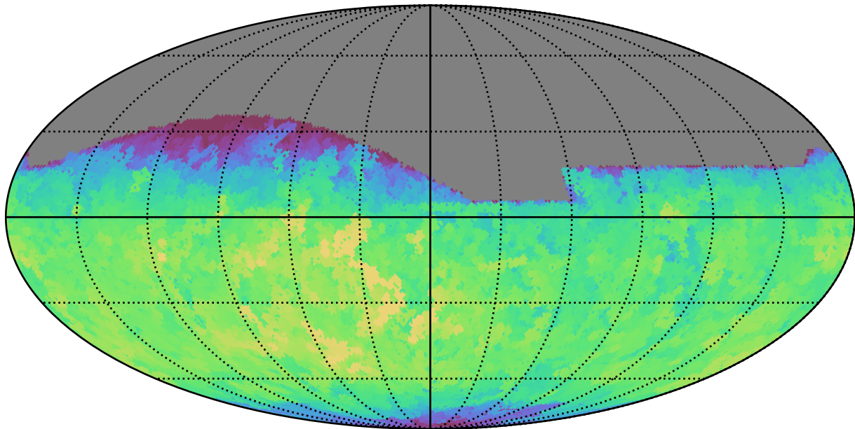
extra_ss_neo7_v3.4_10yrs All sky g band: Max fiveSigmaDepth
