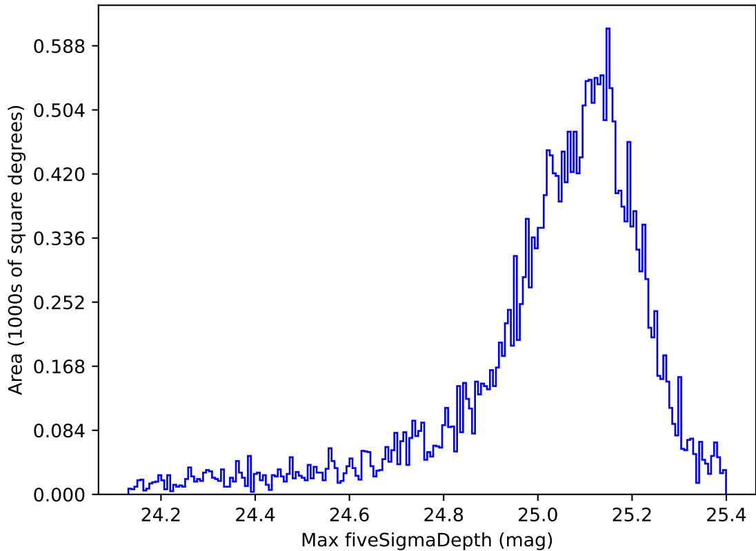
extra_ss_neo7_v3.4_10yrs All sky all bands: Max fiveSigmaDepth
