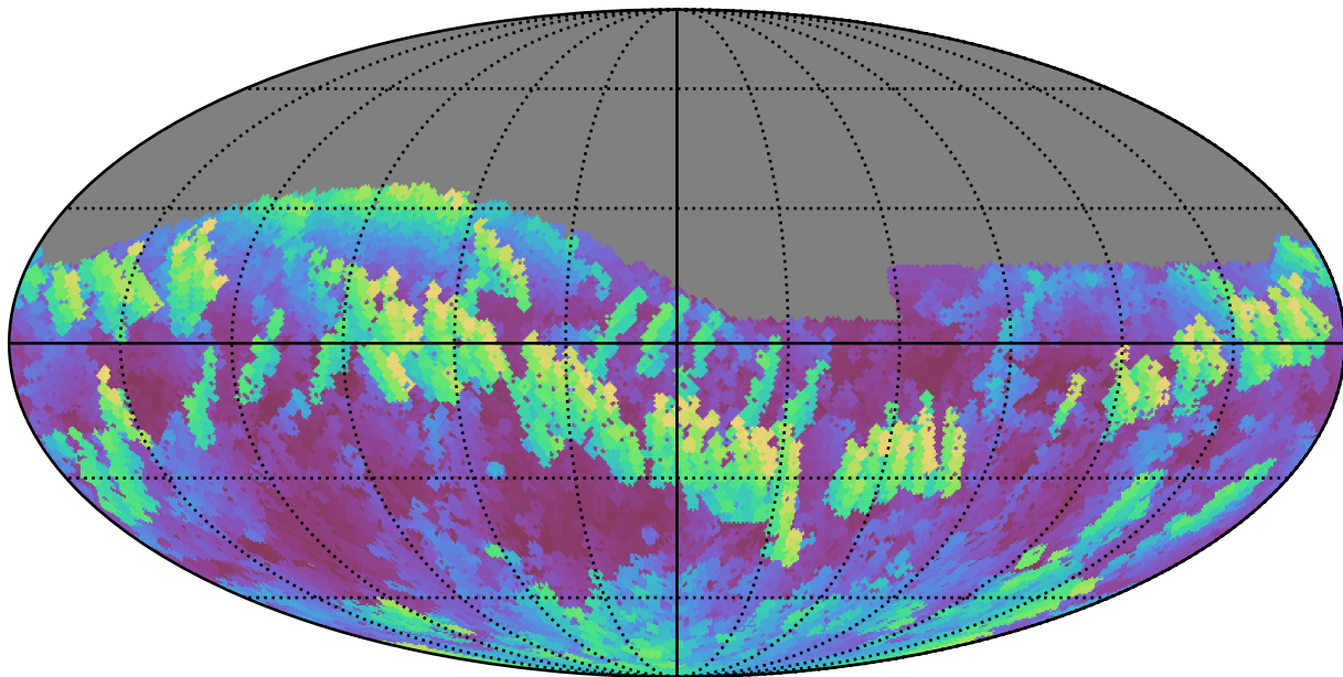
extra_ss_neo7_v3.4_10yrs Yr 1 z band: Max airmass
