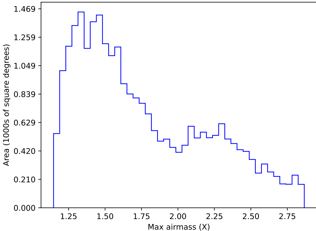
extra_ss_neo7_v3.4_10yrs Yr 1 z band: Max airmass
