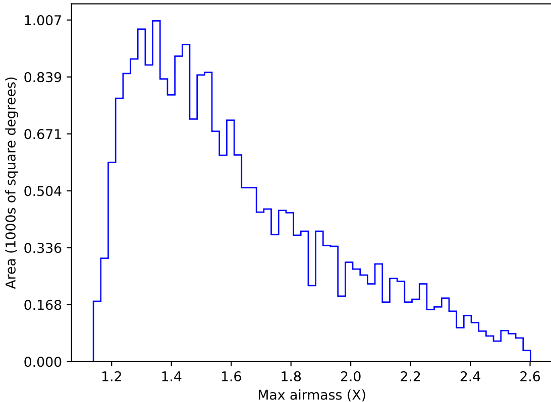
extra_ss_neo7_v3.4_10yrs Yr 1 y band: Max airmass
