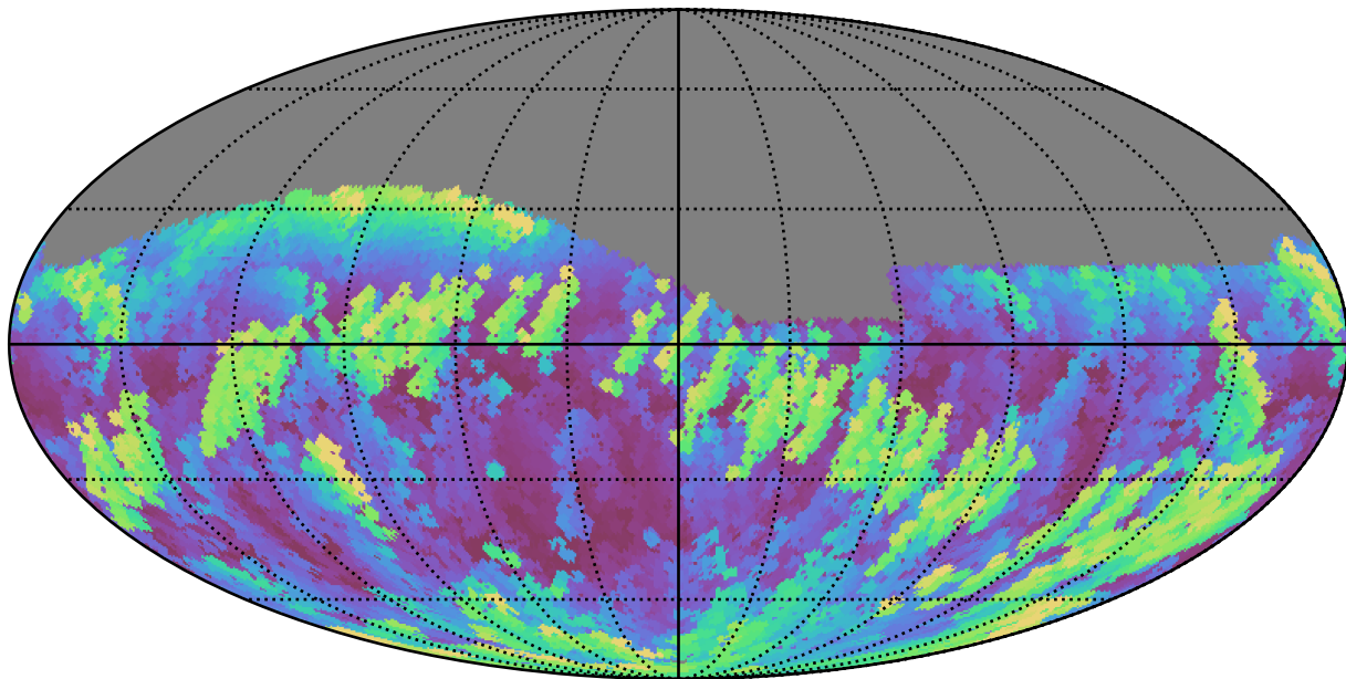
extra_ss_neo7_v3.4_10yrs Yr 1 r band: Max airmass
