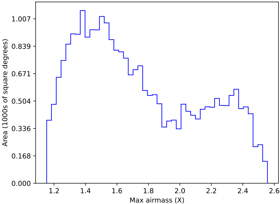
extra_ss_neo7_v3.4_10yrs Yr 1 r band: Max airmass
