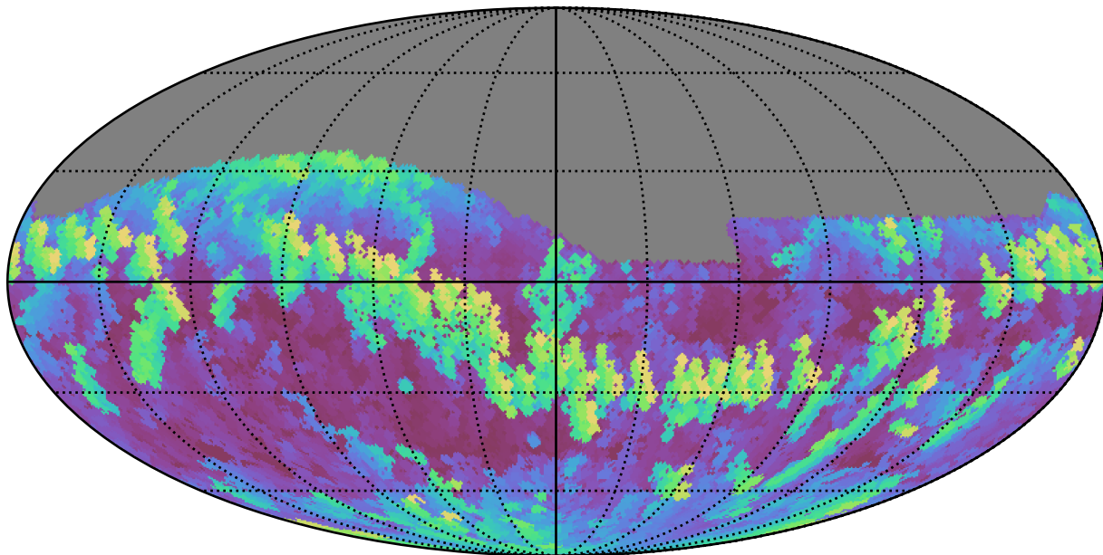
extra_ss_neo7_v3.4_10yrs Yr 1 i band: Max airmass
