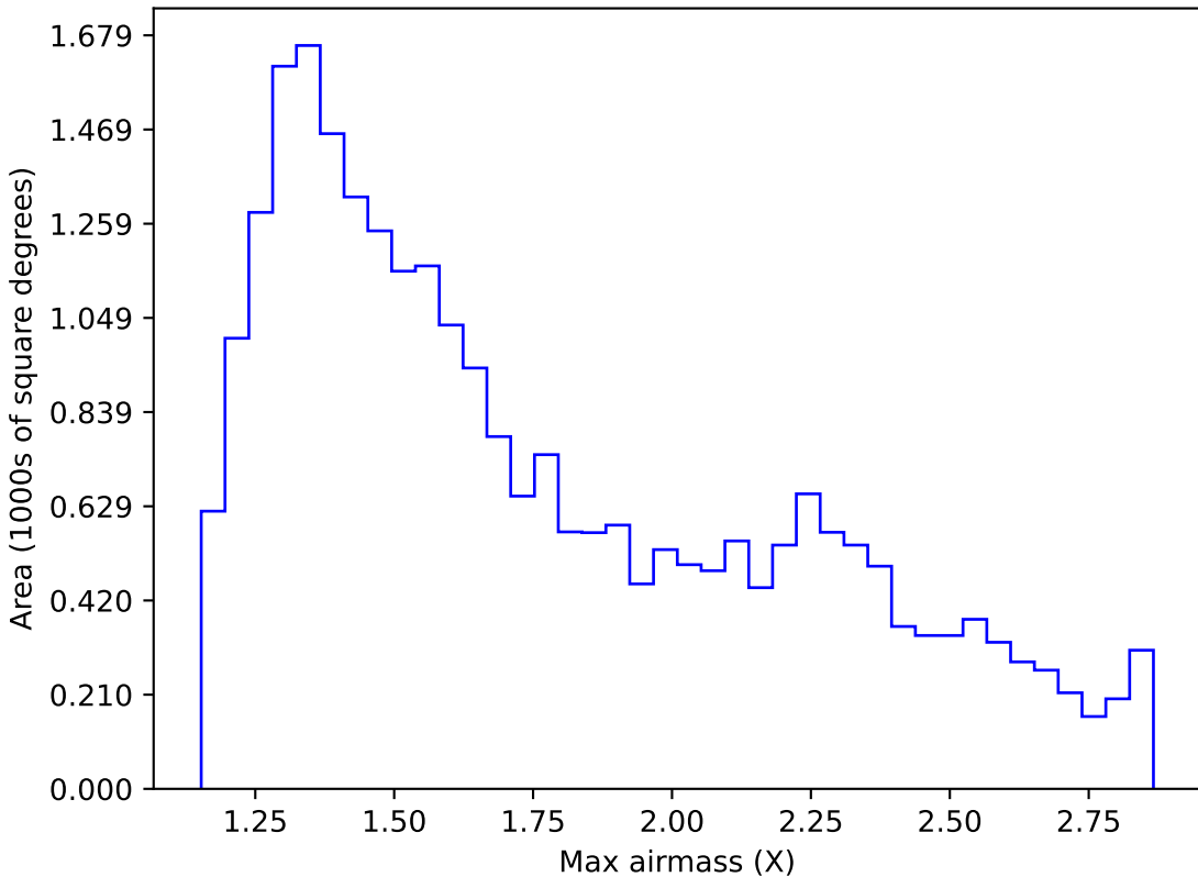
extra_ss_neo7_v3.4_10yrs Yr 1 i band: Max airmass
