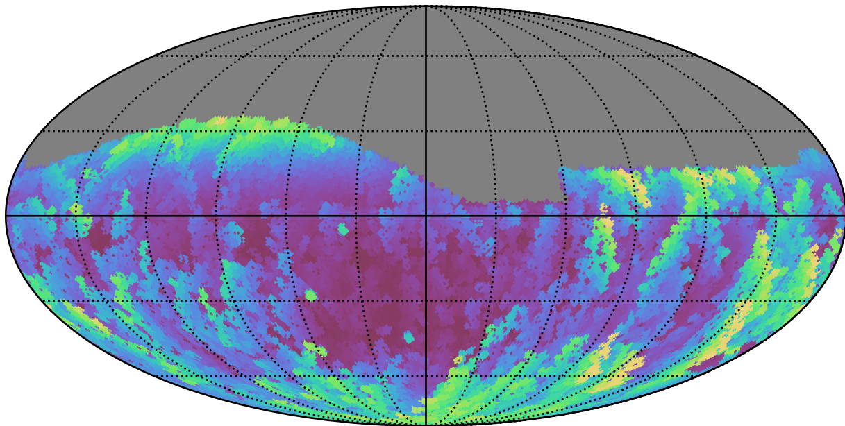
extra_ss_neo7_v3.4_10yrs Yr 1 g band: Max airmass
