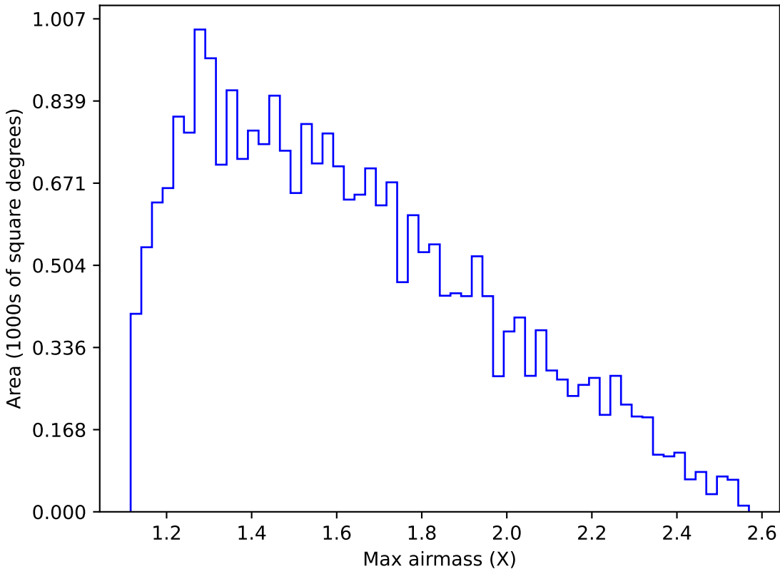
extra_ss_neo7_v3.4_10yrs Yr 1 g band: Max airmass
