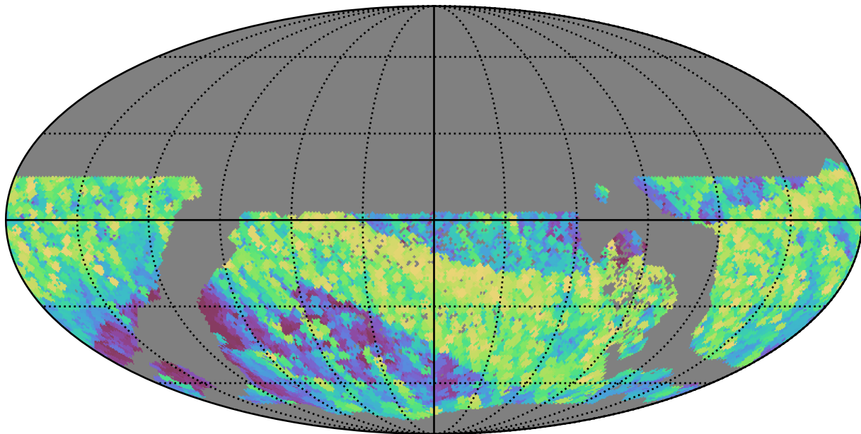
extra_ss_neo7_v3.4_10yrs WFD z band: Max airmass
