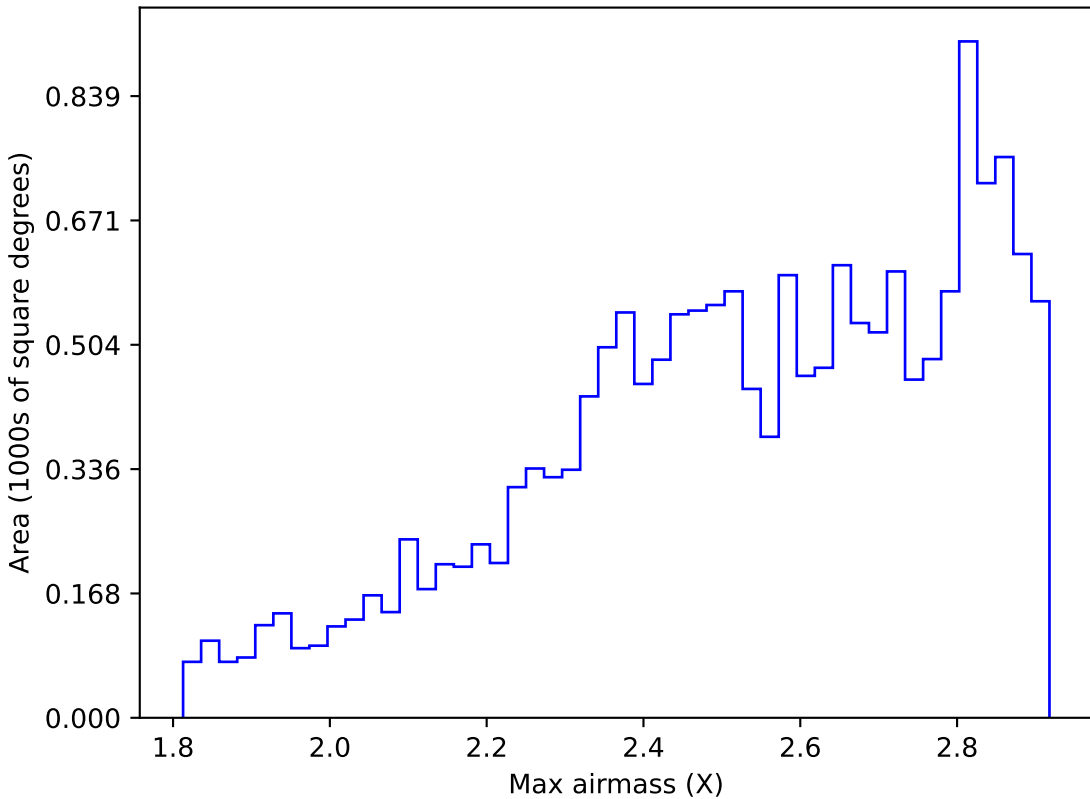
extra_ss_neo7_v3.4_10yrs WFD z band: Max airmass
