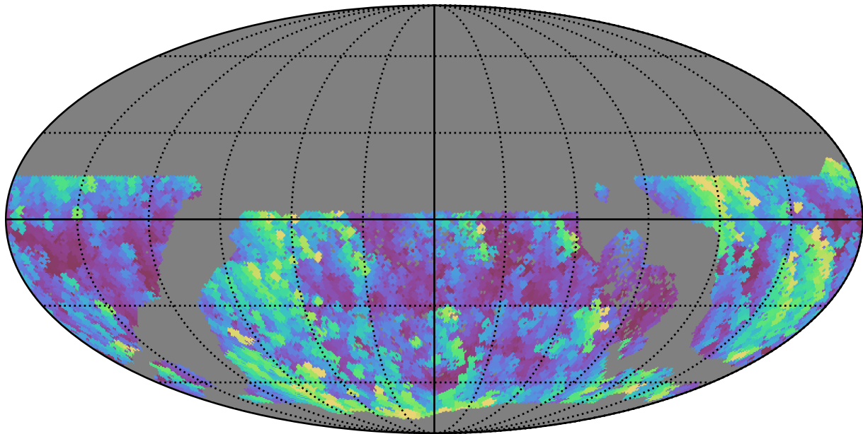
extra_ss_neo7_v3.4_10yrs WFD u band: Max airmass
