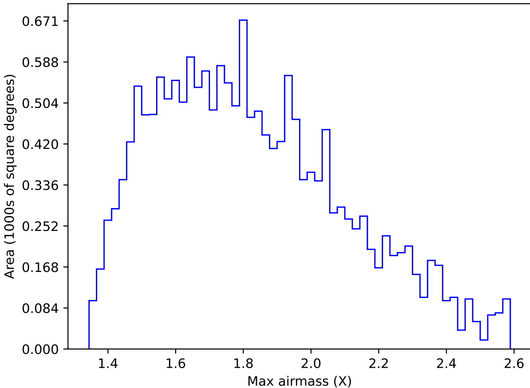
extra_ss_neo7_v3.4_10yrs WFD u band: Max airmass
