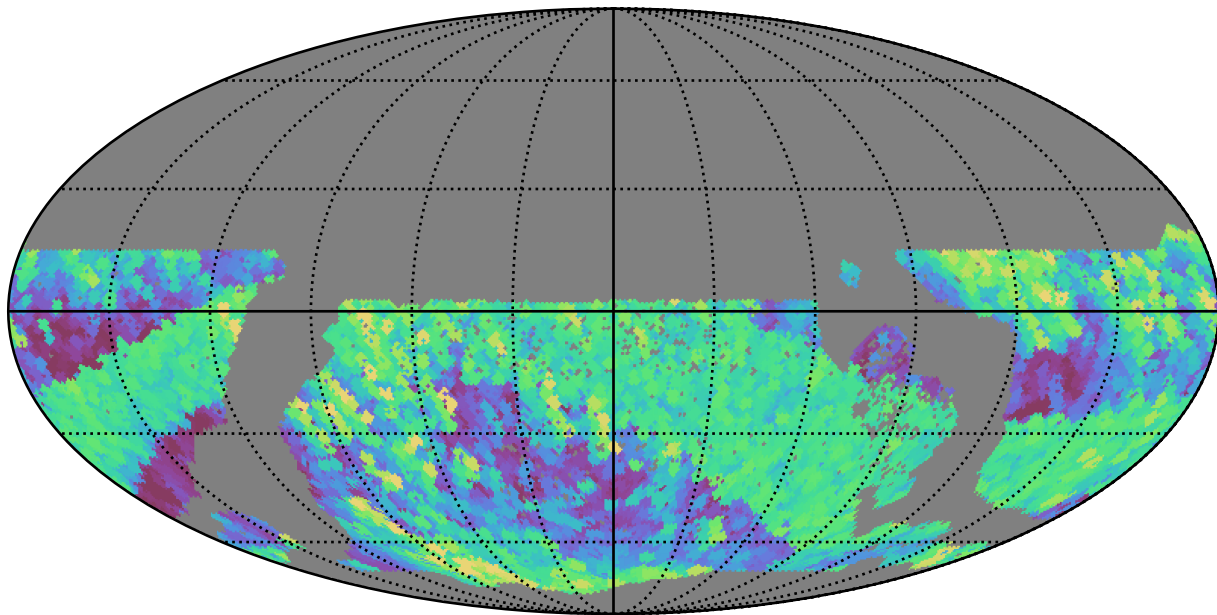
extra_ss_neo7_v3.4_10yrs WFD r band: Max airmass
