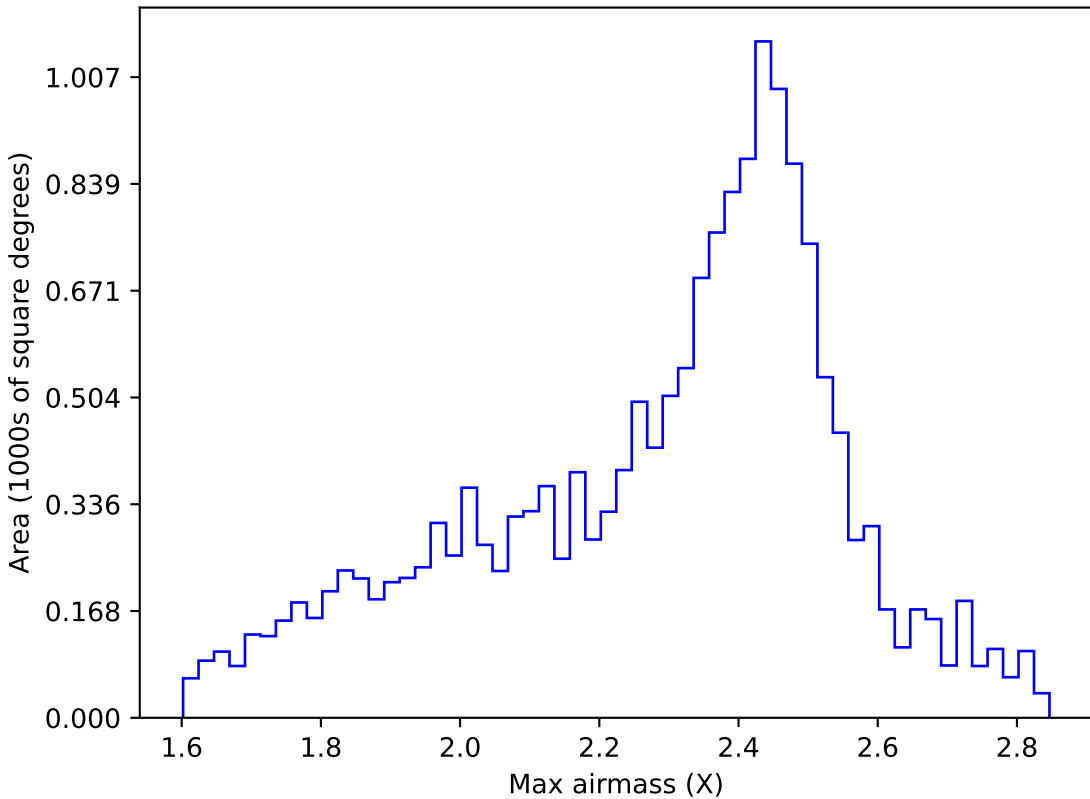
extra_ss_neo7_v3.4_10yrs WFD r band: Max airmass
