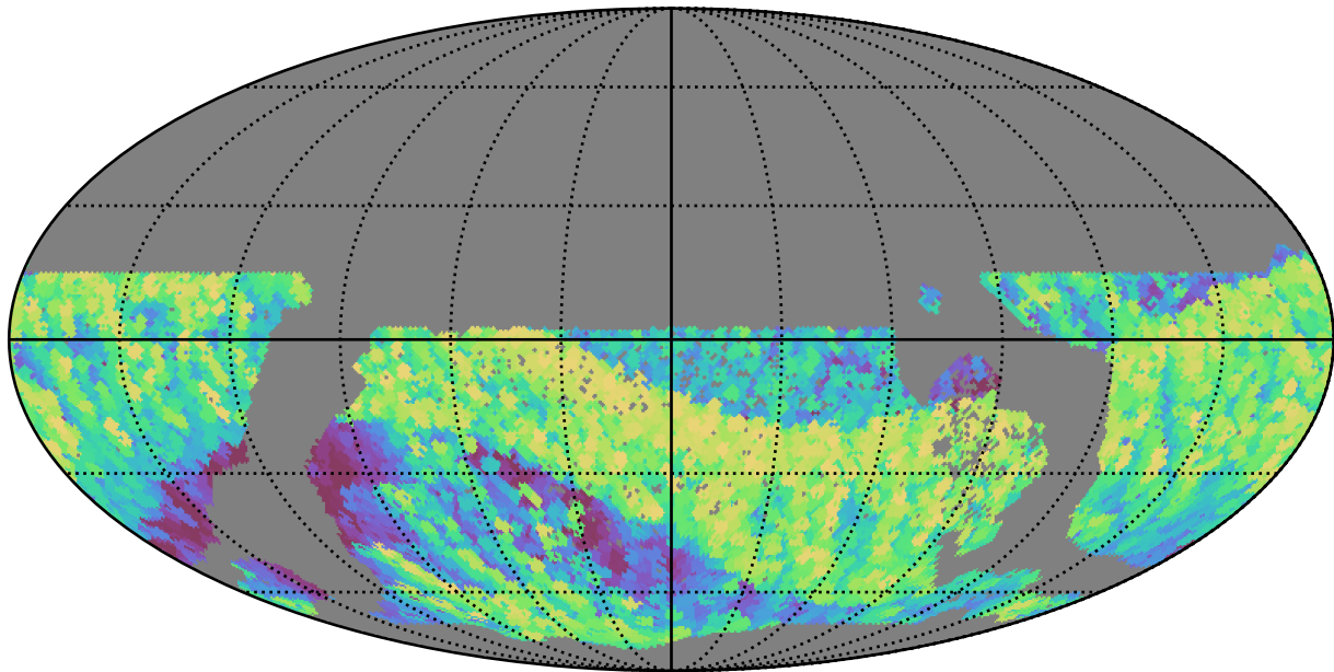
extra_ss_neo7_v3.4_10yrs WFD i band: Max airmass
