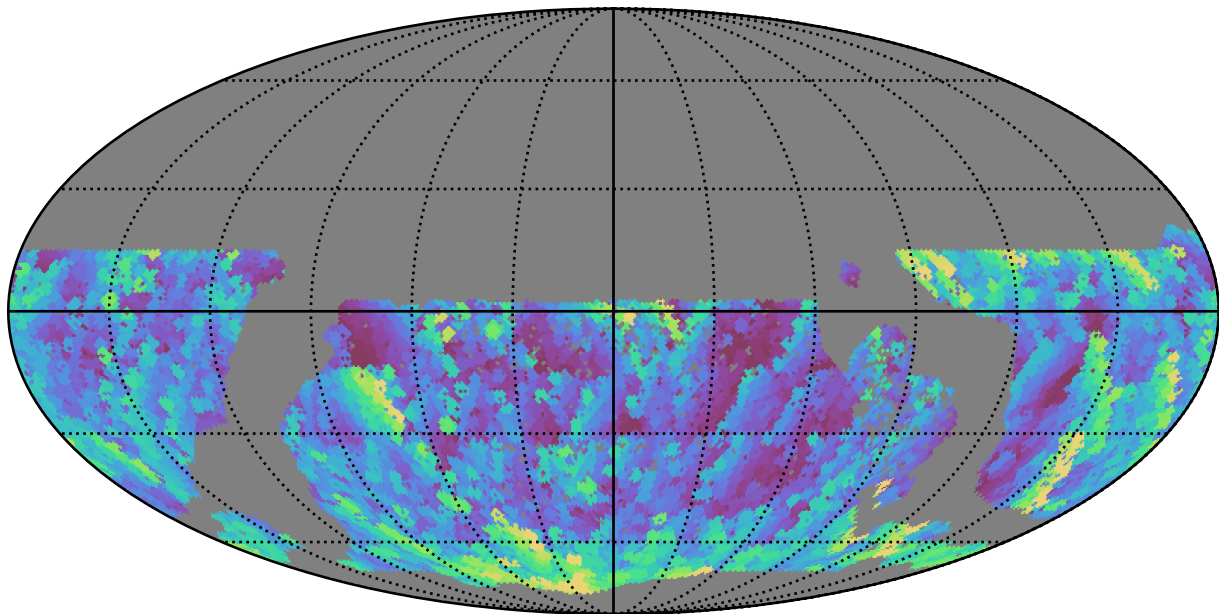
extra_ss_neo7_v3.4_10yrs WFD g band: Max airmass
