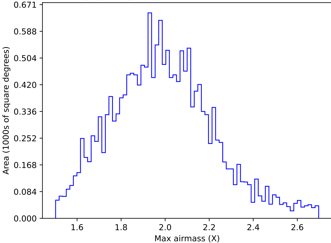
extra_ss_neo7_v3.4_10yrs WFD g band: Max airmass
