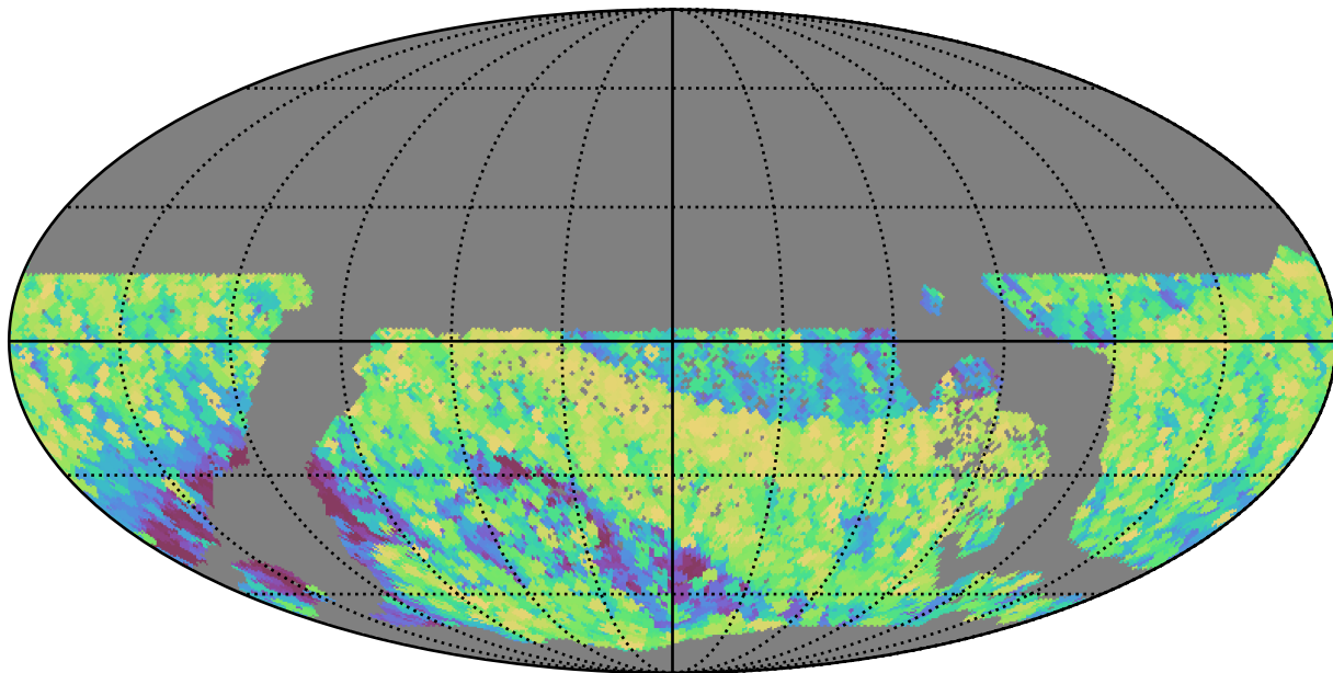
extra_ss_neo7_v3.4_10yrs WFD all bands: Max airmass
