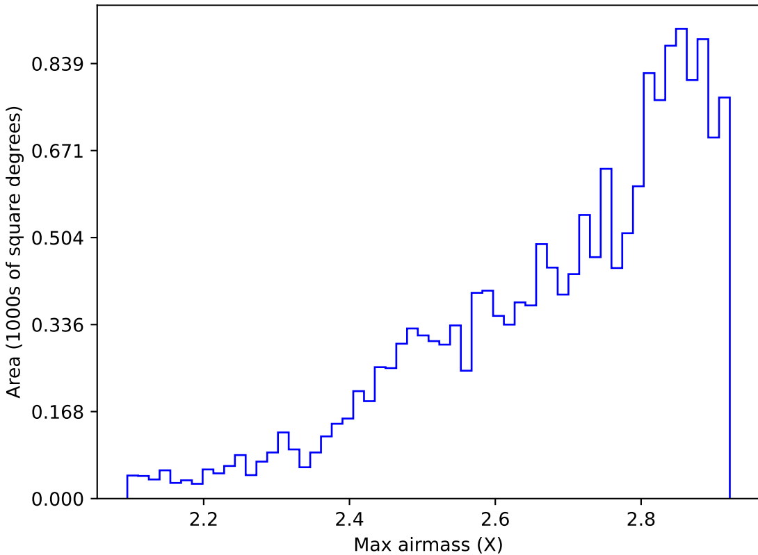
extra_ss_neo7_v3.4_10yrs WFD all bands: Max airmass
