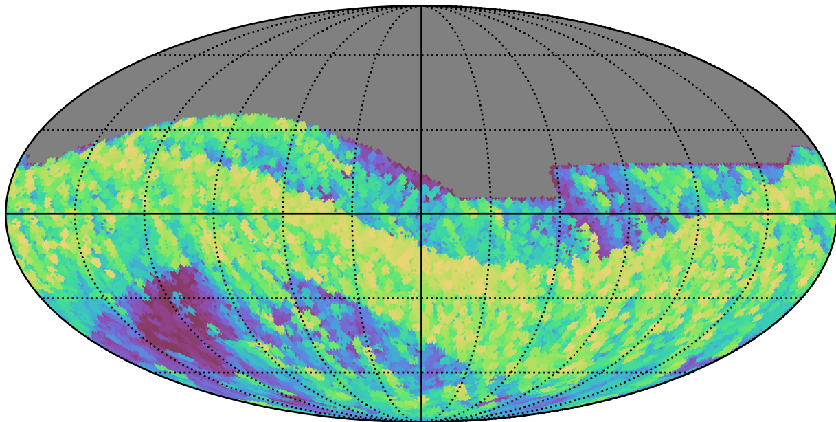
extra_ss_neo7_v3.4_10yrs All sky z band: Max airmass
