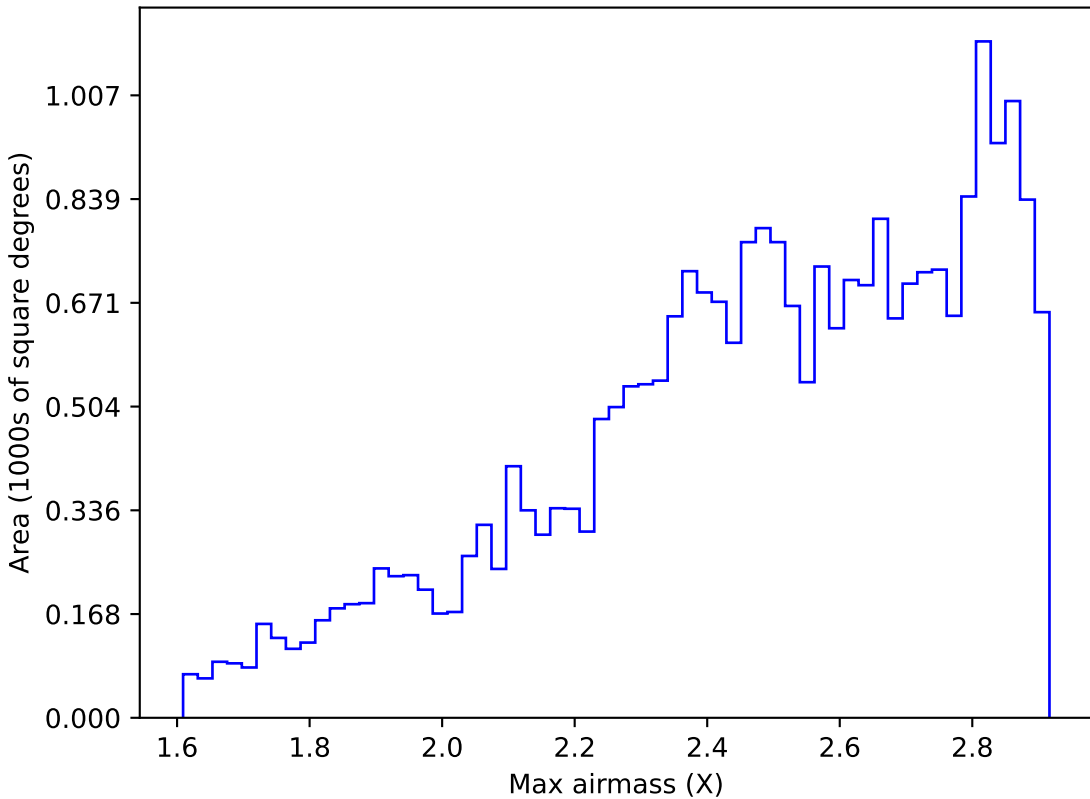
extra_ss_neo7_v3.4_10yrs All sky z band: Max airmass
