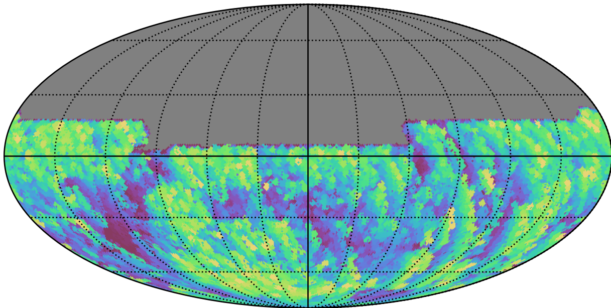
extra_ss_neo7_v3.4_10yrs All sky y band: Max airmass
