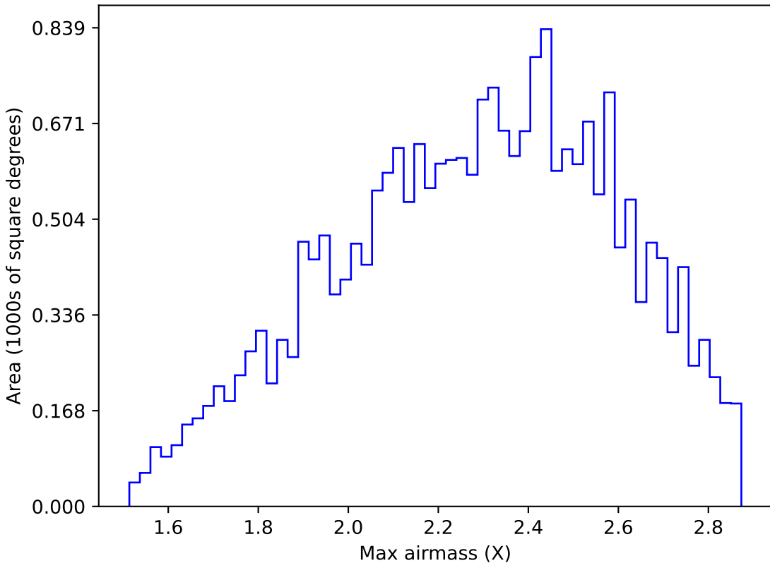
extra_ss_neo7_v3.4_10yrs All sky y band: Max airmass
