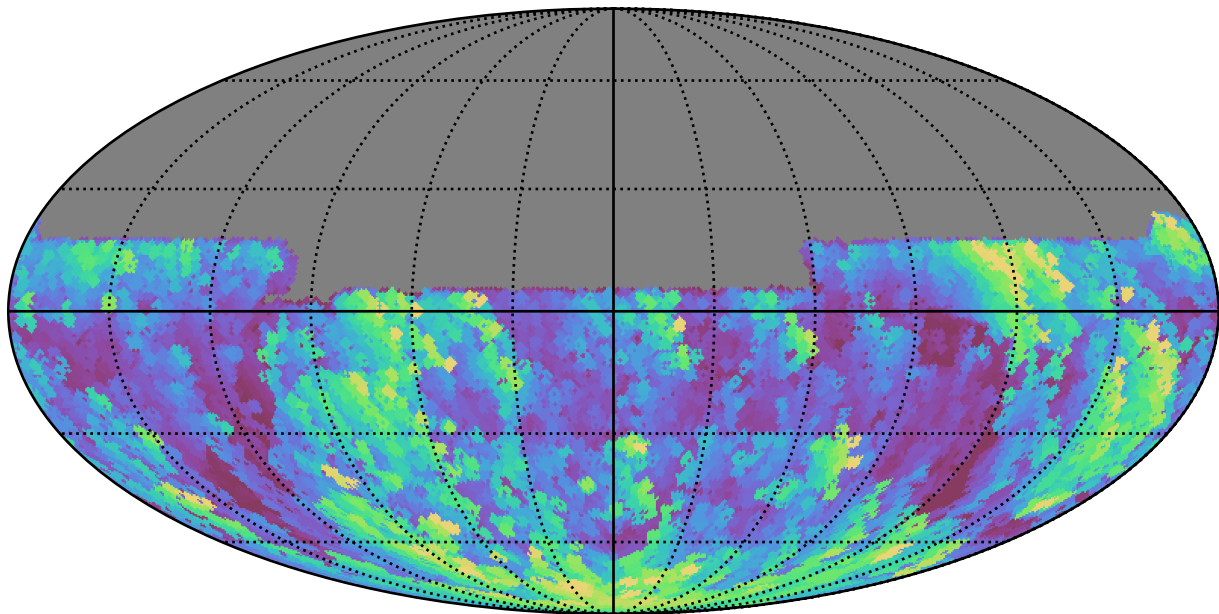
extra_ss_neo7_v3.4_10yrs All sky u band: Max airmass
