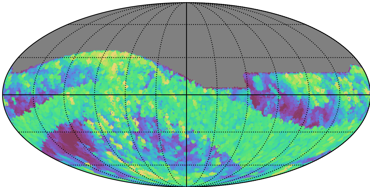
extra_ss_neo7_v3.4_10yrs All sky r band: Max airmass
