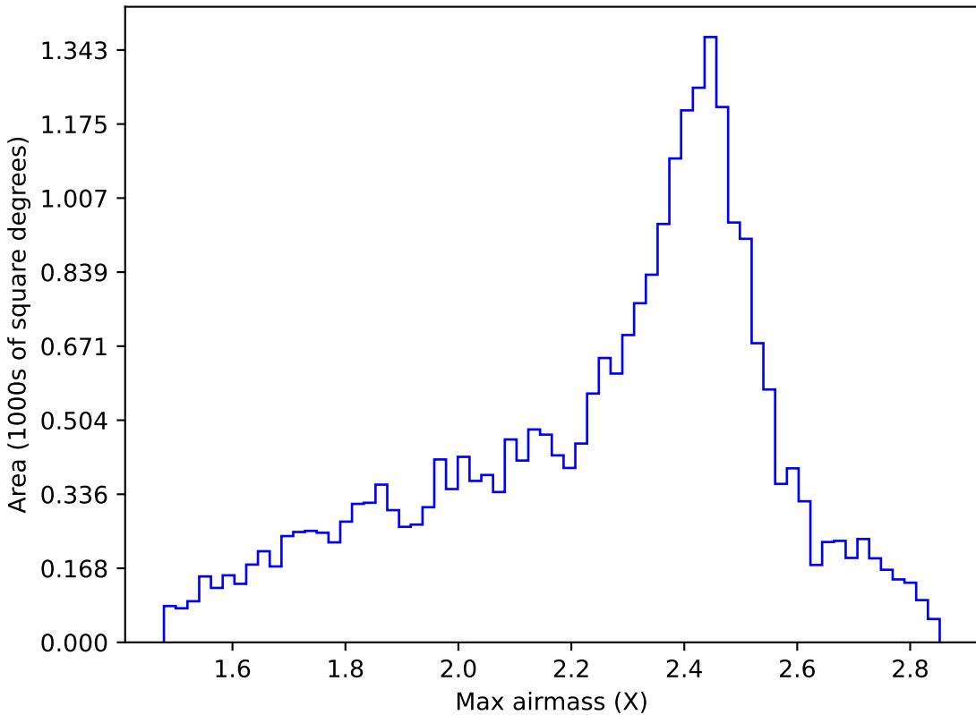
extra_ss_neo7_v3.4_10yrs All sky r band: Max airmass
