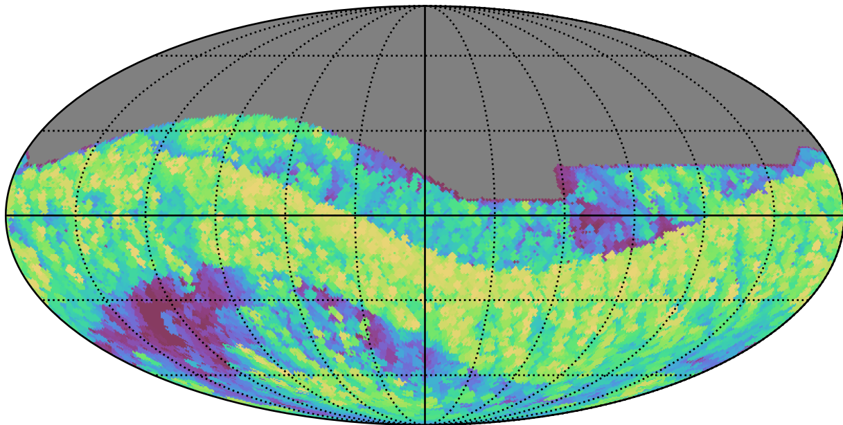
extra_ss_neo7_v3.4_10yrs All sky i band: Max airmass
