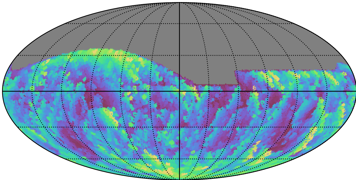
extra_ss_neo7_v3.4_10yrs All sky g band: Max airmass
