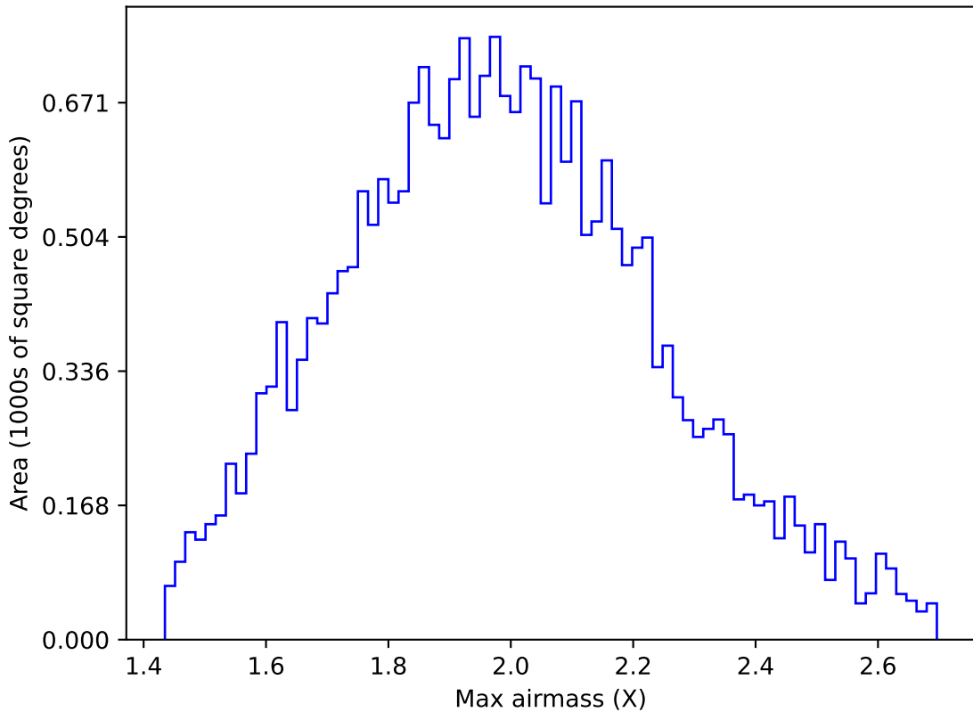
extra_ss_neo7_v3.4_10yrs All sky g band: Max airmass
