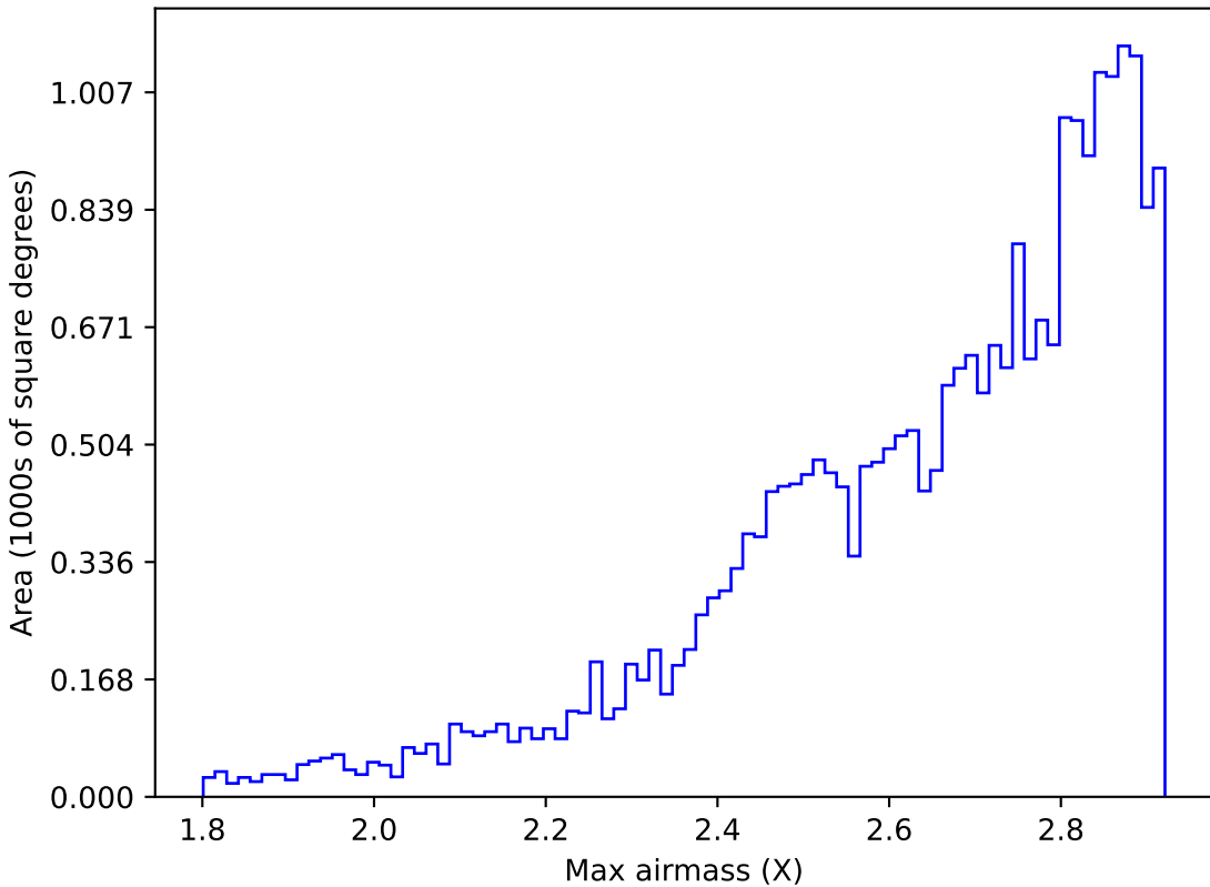
extra_ss_neo7_v3.4_10yrs All sky all bands: Max airmass
