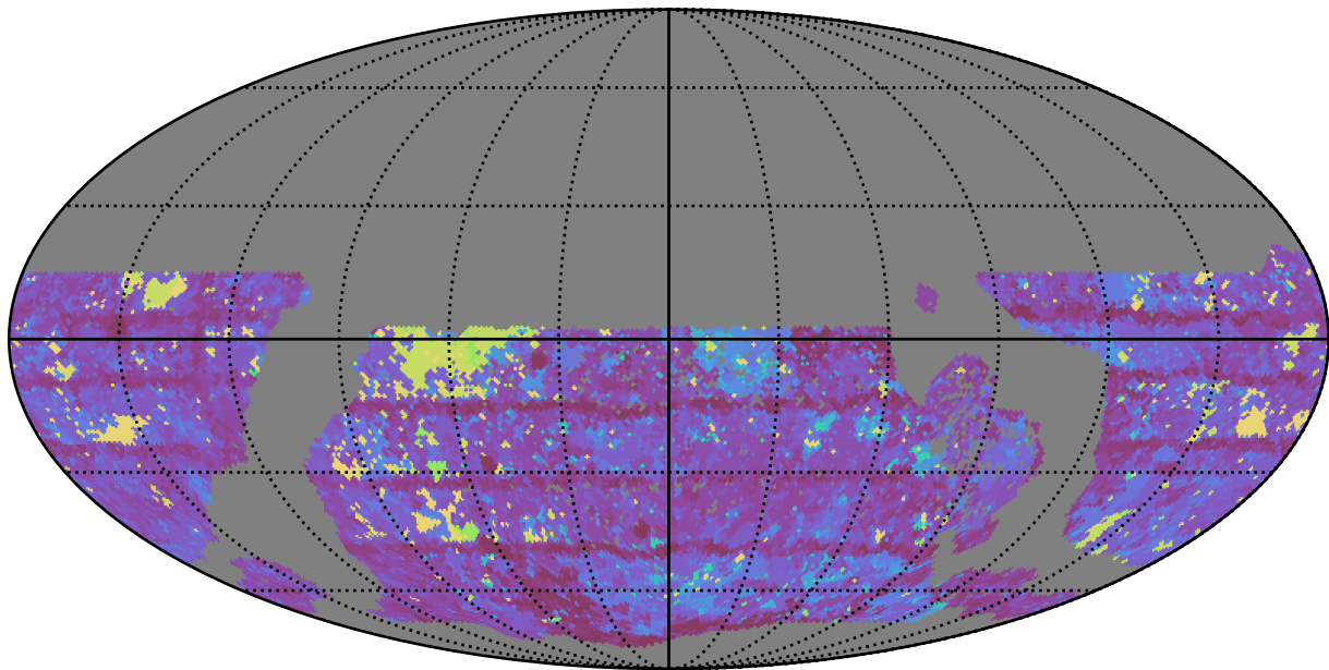
extra_ss_neo7_v3.4_10yrs WFD y band: Max Inter-Night Gap
