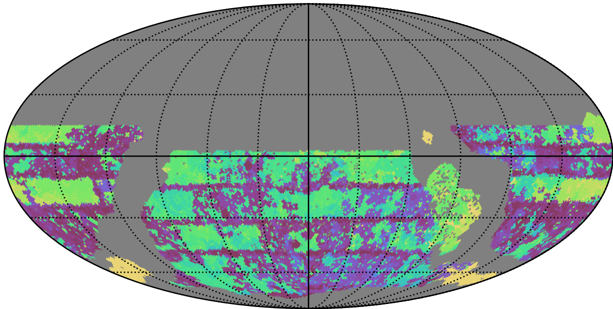
extra_ss_neo7_v3.4_10yrs WFD u band: Max Inter-Night Gap
