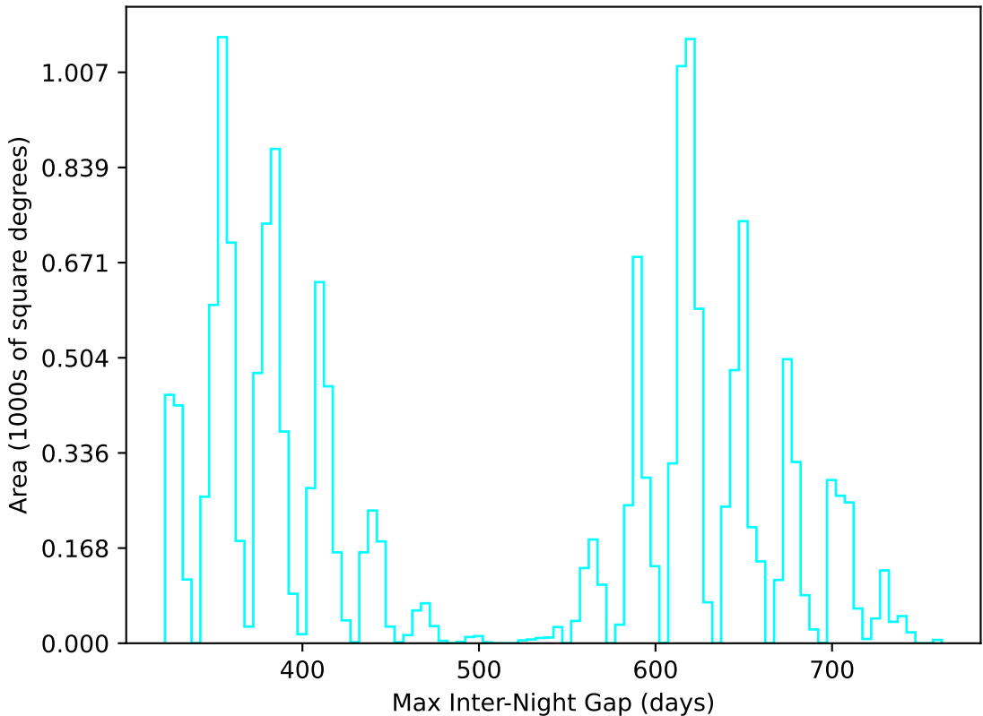
extra_ss_neo7_v3.4_10yrs WFD u band: Max Inter-Night Gap
