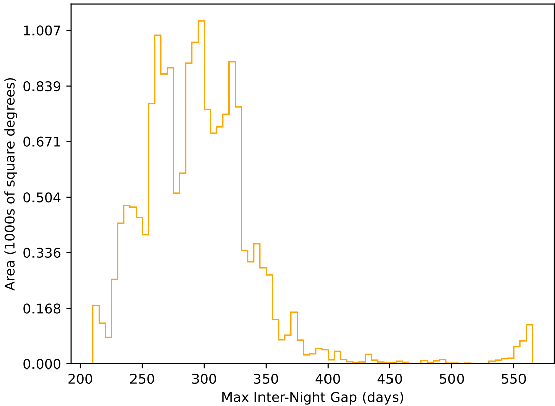
extra_ss_neo7_v3.4_10yrs WFD r band: Max Inter-Night Gap
