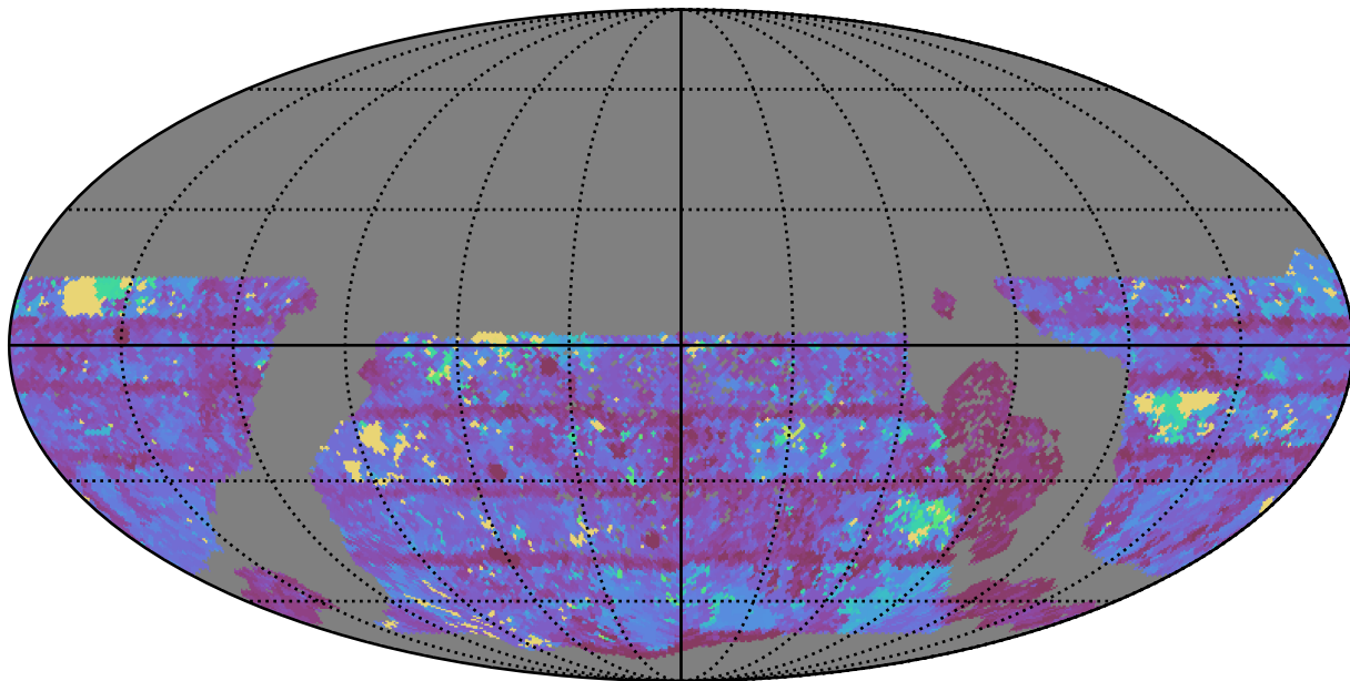
extra_ss_neo7_v3.4_10yrs WFD i band: Max Inter-Night Gap
