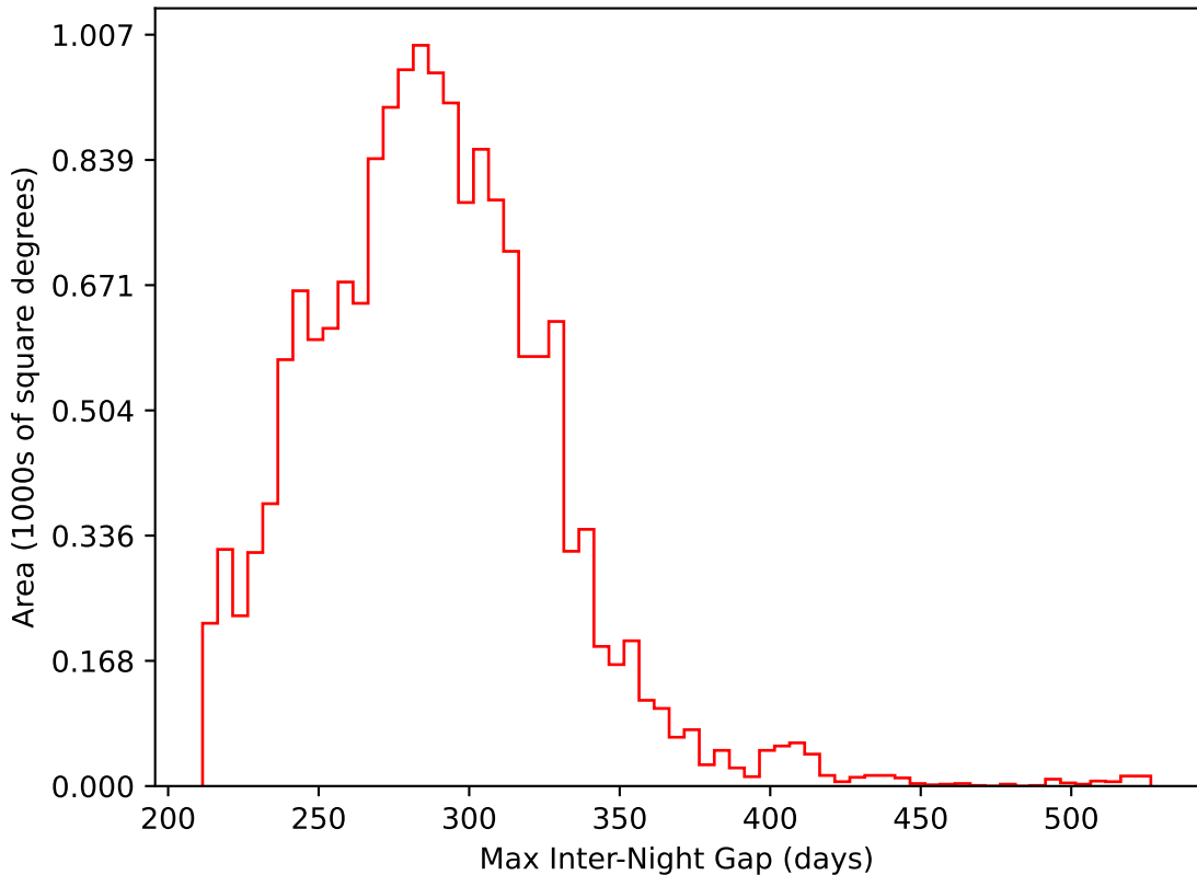
extra_ss_neo7_v3.4_10yrs WFD i band: Max Inter-Night Gap
