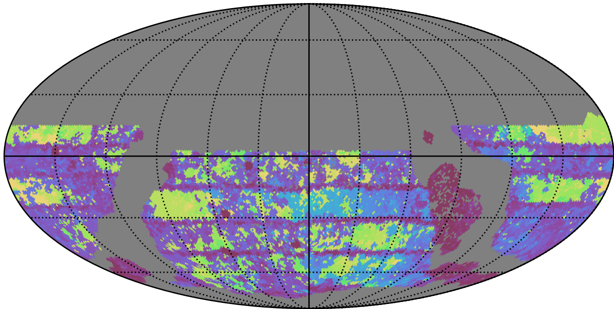
extra_ss_neo7_v3.4_10yrs WFD g band: Max Inter-Night Gap
