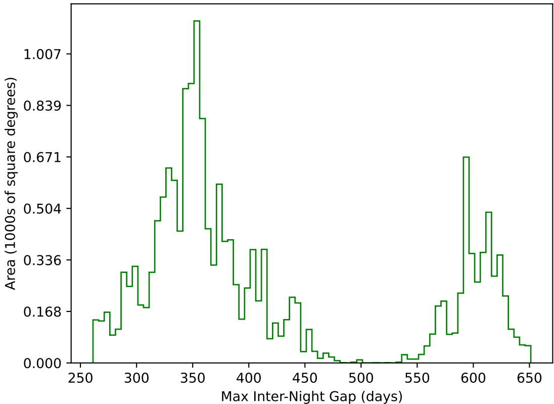
extra_ss_neo7_v3.4_10yrs WFD g band: Max Inter-Night Gap
