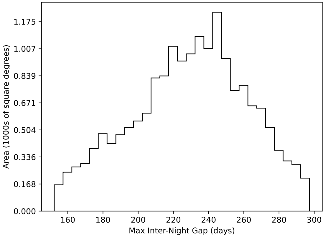
extra_ss_neo7_v3.4_10yrs WFD all bands: Max Inter-Night Gap
