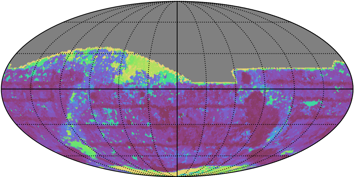
extra_ss_neo7_v3.4_10yrs All sky z band: Max Inter-Night Gap
