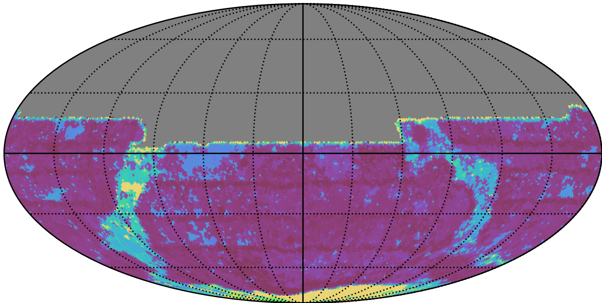
extra_ss_neo7_v3.4_10yrs All sky y band: Max Inter-Night Gap
