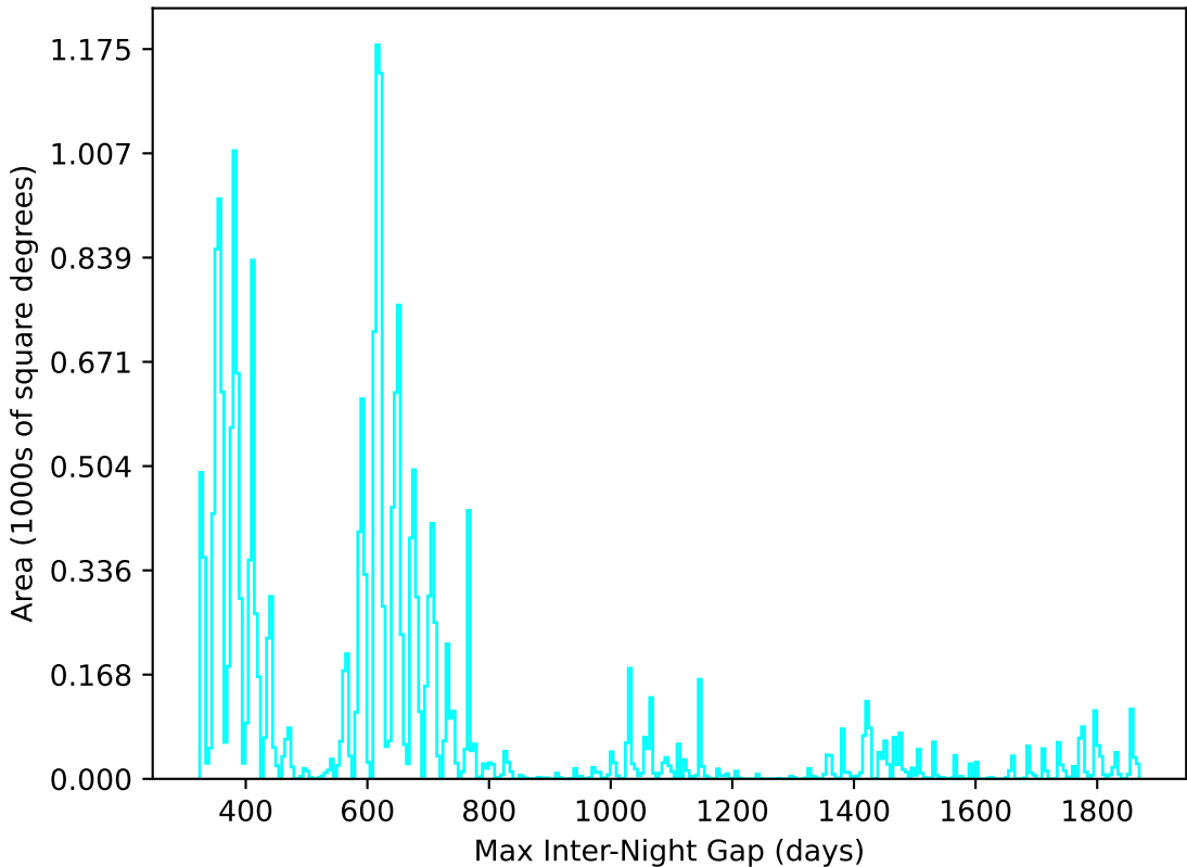
extra_ss_neo7_v3.4_10yrs All sky u band: Max Inter-Night Gap
