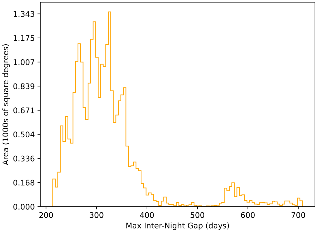
extra_ss_neo7_v3.4_10yrs All sky r band: Max Inter-Night Gap
