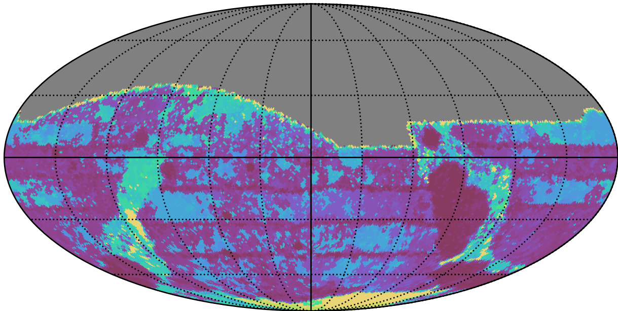
extra_ss_neo7_v3.4_10yrs All sky g band: Max Inter-Night Gap
