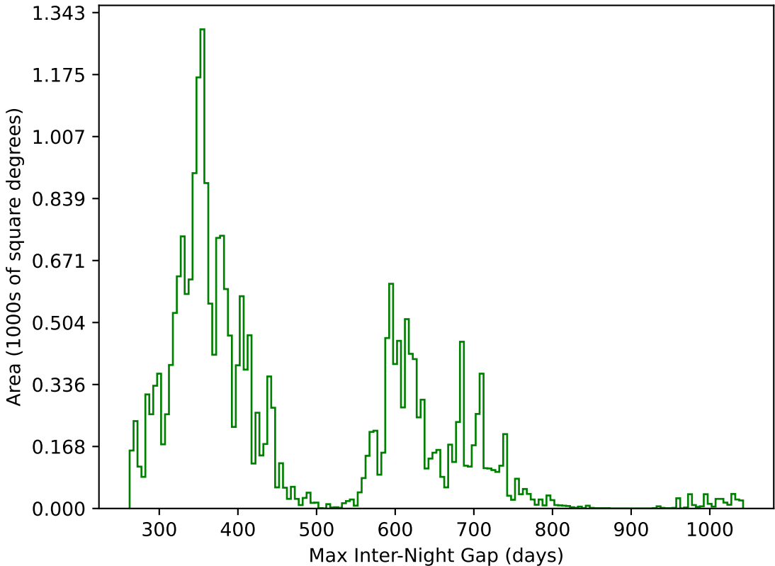
extra_ss_neo7_v3.4_10yrs All sky g band: Max Inter-Night Gap
