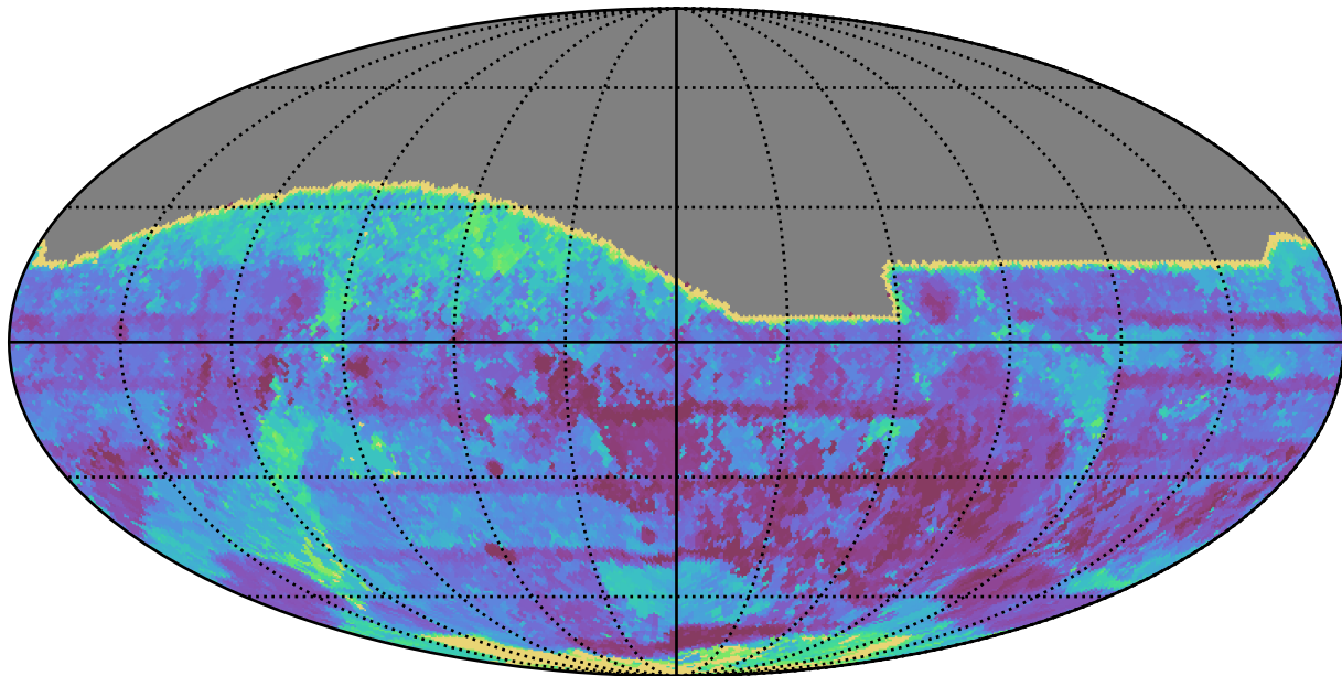
extra_ss_neo7_v3.4_10yrs All sky all bands: Max Inter-Night Gap
