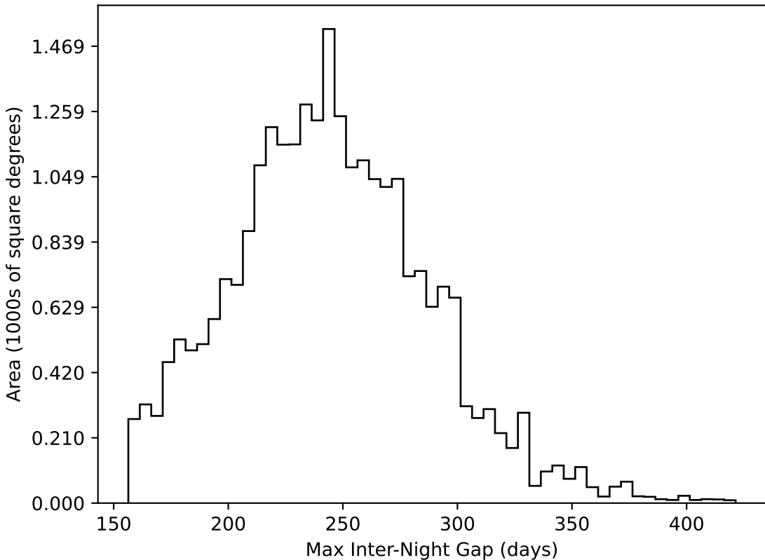
extra_ss_neo7_v3.4_10yrs All sky all bands: Max Inter-Night Gap
